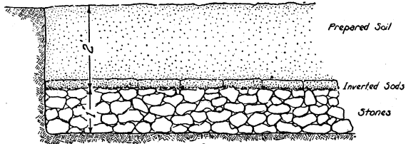
FIGURE 3.—A bed specially prepared for plant growth where the normal drainage is inadequate
